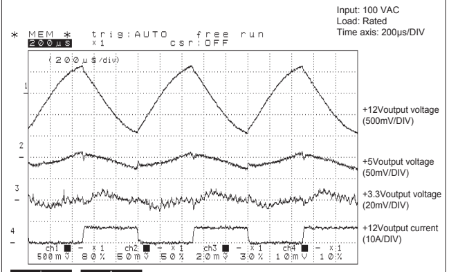
• Fig.14 Dynamic Load Fluctuation Characteristics at 1kHz
