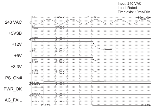
• Fig.12 Falling Characteristics at 240 VAC when REMOTE goes Off
