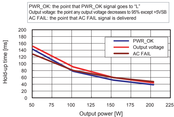
• Fig.13 Output Hold-up Time vs. Output Power
