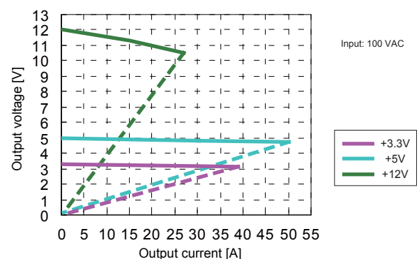
• Fig.18 Over Current Protection (V-I Characteristic)
