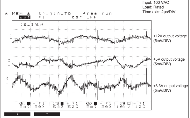
• Fig.16 Ripple and Spike Voltage
