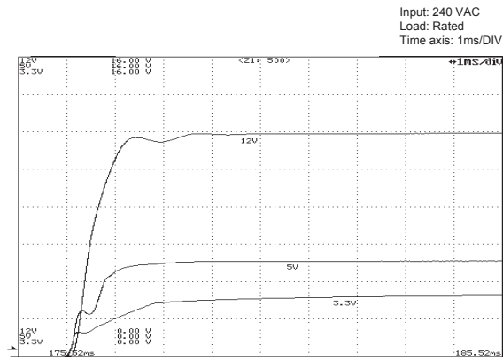
• Fig.11 Rising Characteristics at 240 VAC
